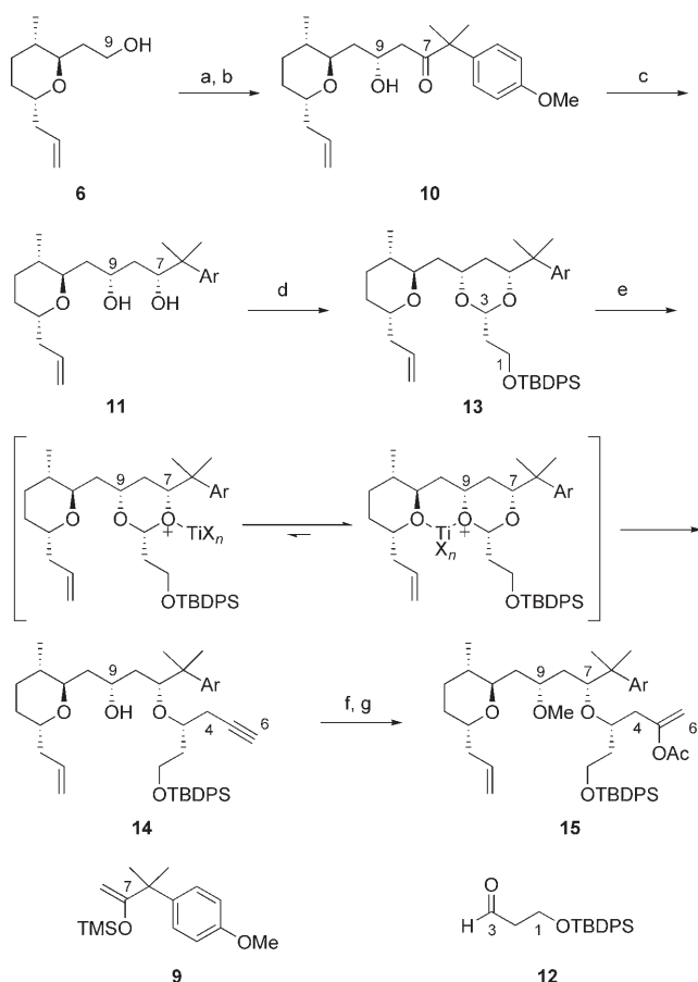
Scheme 3. ETIC substrate synthesis. a) Dess–Martin periodinane, pyridine, \text{CH}_2\text{Cl}_2 , -78^\circ\text{C} , 78% yield (two steps), d.r. = 4.5:1. c) \text{NaBH}_4 , \text{Et}_2\text{BOMe} , MeOH, THF, then NaOAc, 76% yield. d) 1) TMSOTf, 2,6-lutidine, \text{CH}_2\text{Cl}_2 , -78^\circ\text{C} , 87% yield. 2) 12 , TMSOTf, \text{CH}_2\text{Cl}_2 , -78 – -45^\circ\text{C} , 87% yield. e) Allenyltributyltin, \text{TiCl}_4/\text{Ti}(\text{O}i\text{Pr})_4 (3:1), \text{CH}_2\text{Cl}_2 , -78^\circ\text{C} , 89% yield. f) MeOTf, 2,6-di- tert -butylpyridine, \text{CH}_2\text{Cl}_2 , 87% yield. g) HOAc, [\text{Ru}(\text{p-cymene})\text{Cl}]_2 , (2-furyl) _3\text{P} , \text{Na}_2\text{CO}_3 , toluene, 72% yield. TBDPS = tert -butyldiphenylsilyl, TMS = trimethylsilyl, Tf = trifluoromethanesulfonyl.
